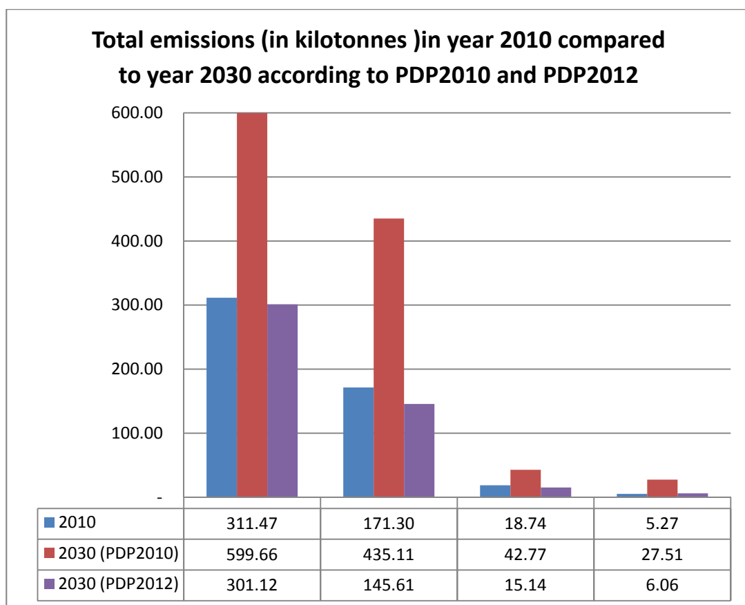
Figure 6: Comparison of PDP2010 and PDP2012 on total nitrogen-oxides (NOx), sulfurdioxide (SO2), total suspended particulates (TSP) and mercury (Hg) emissions in year 2010 and 2030.
